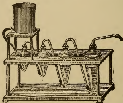
Fig. 99. APPARATUS FOR ANALYZING THE SOIL.
